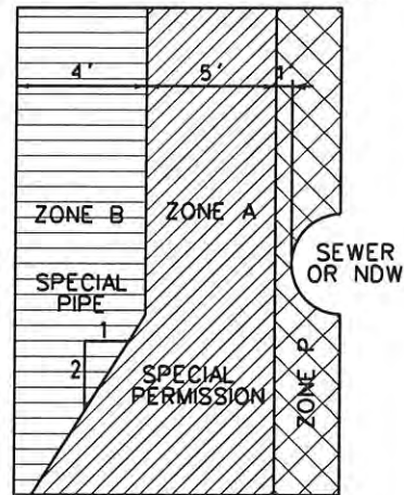
PARALLEL CONSTRUCTION
