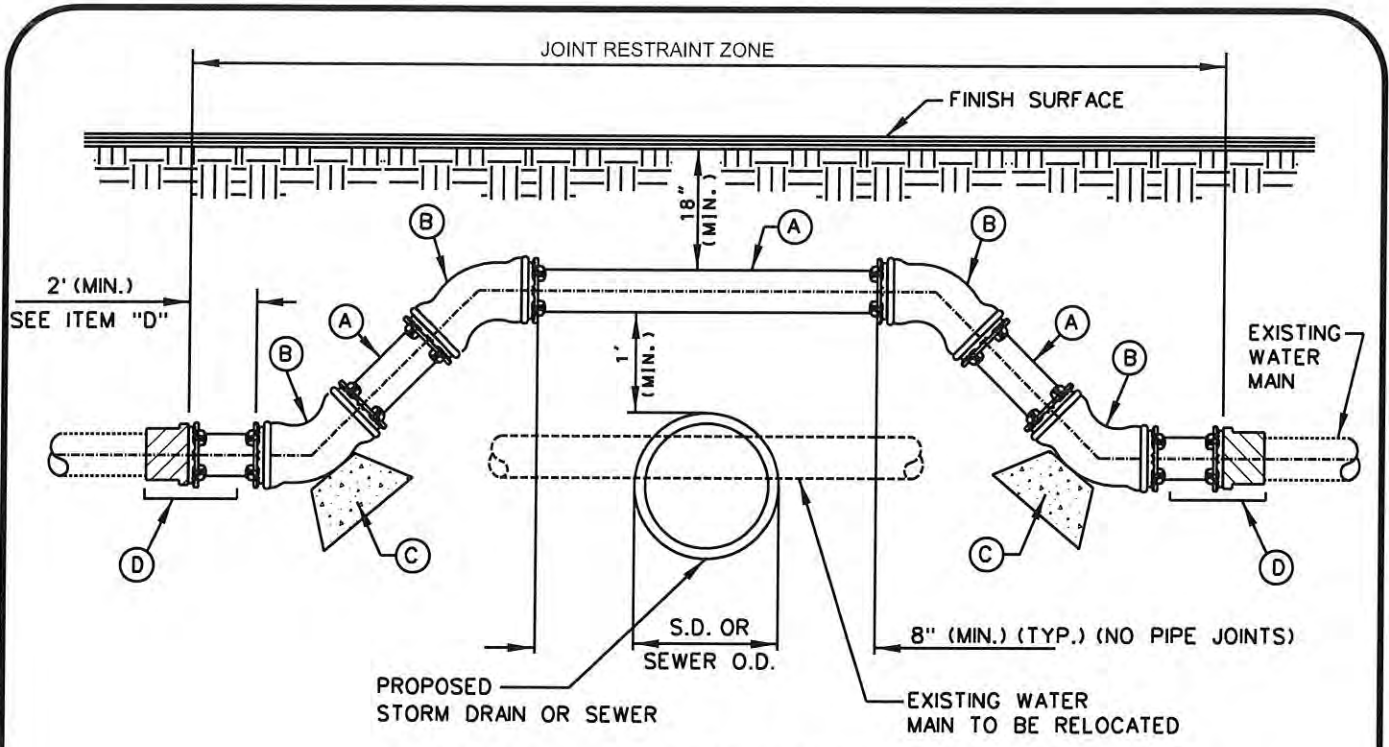
TYPE 1- VERTICAL OFFSET PROFILE
