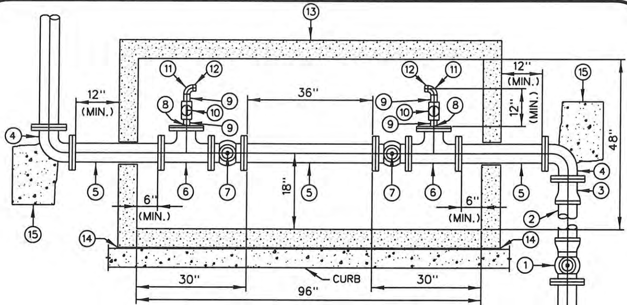
PLAN VIEW
