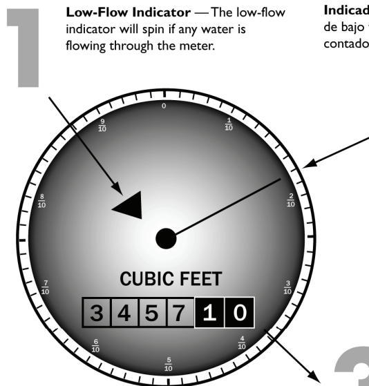
Meter Register — The meter register is a lot like the mileage odometer on your car. The numbers keep a running total of all the water that has passed through the meter. The register shown here indicates that 345,710 cubic feet of water has passed through this meter.
